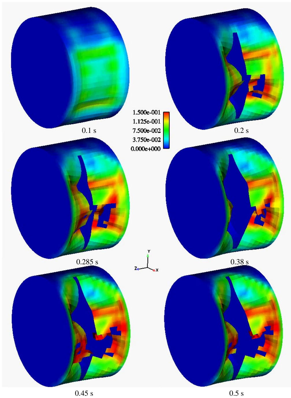
Fig. 6b Effective plastic strain plotted on the deformed shapes of the cylinder
