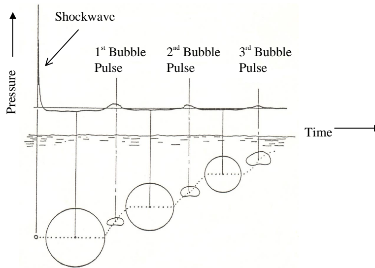
Fig. 1 Pressure waves and bubble phenomena of UNDEX
