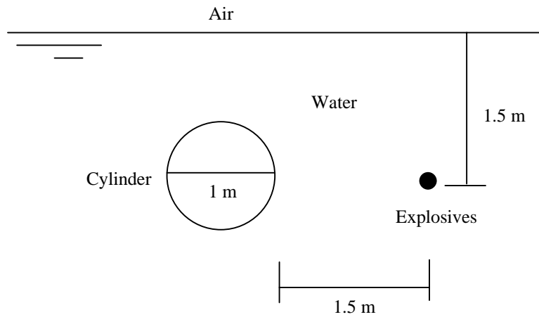
Fig. 2 Positions of cylinder, water surface and explosive
