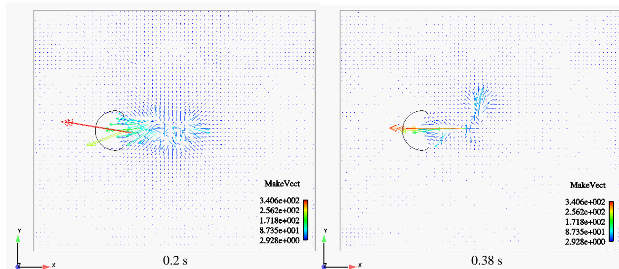
Fig. 7 Velocity distribution of fluid
