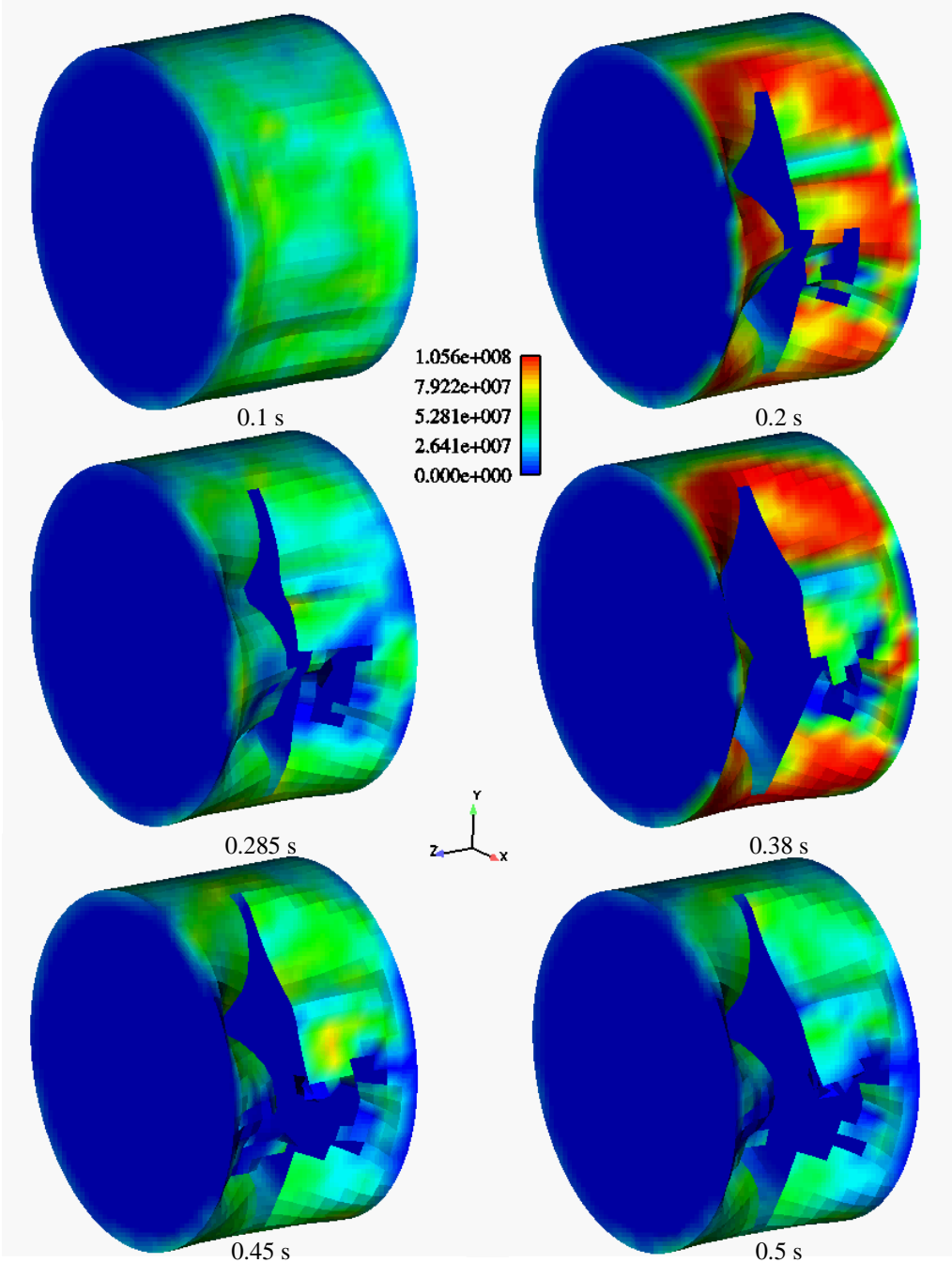
Fig. 6a Effective stress plotted on the deformed shapes of the cylinder
